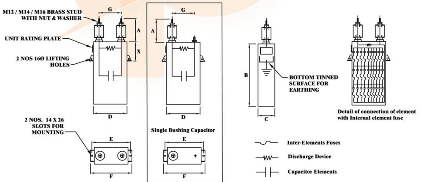
Single Phase Two Bushing Capacitor
